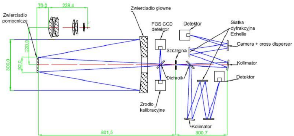
Fig. 2: Generic simultaneous spectroscopic and photometric scheme
